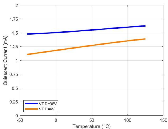
Fig.7-2. Quiescent Current vs. Temperature, 1-Channel OPA
