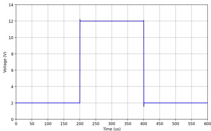
Fig.7-3. 12-V Signal Step Response
