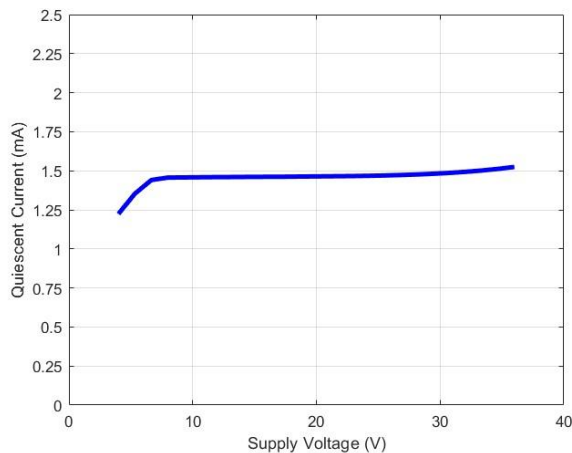
Fig.7-1. Quiescent Current vs. Supply Voltage, 1 Channel OPA
