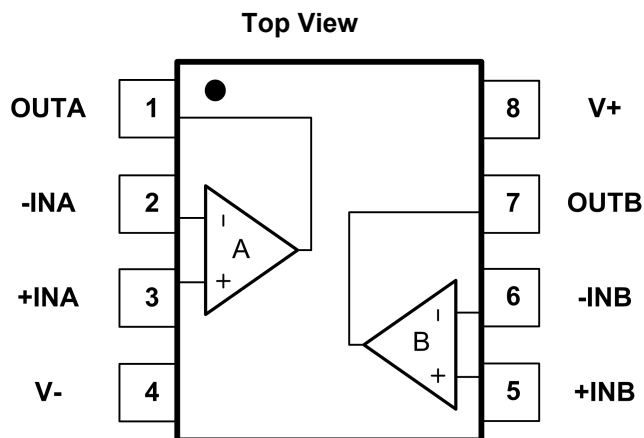
Fig.4-2. GT8442: P8(SOP8) Package GT8442: M8(MSOP8) Package
