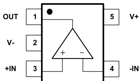
Fig.4-2. GT8391B: S5 (SOT23-5) Package GT8391B: C5 (SC70-5) Package
