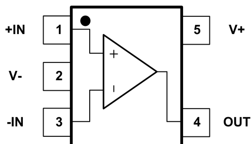
Fig.4-1. GT8391: C5 (SC70-5) Package GT8391: S5 (SOT23-5) Package
