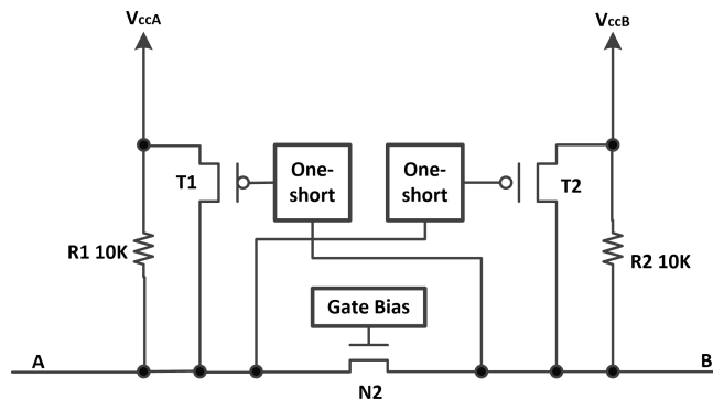
Fig.9-1. Architecture of GT0104
