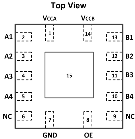
Fig.4-1. GT0104: QD (QFN3.5×3.5-14L) Package
