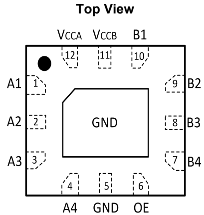
Fig.4-2. GT0104: SC (QFN2.0×2.0-12L) Package
