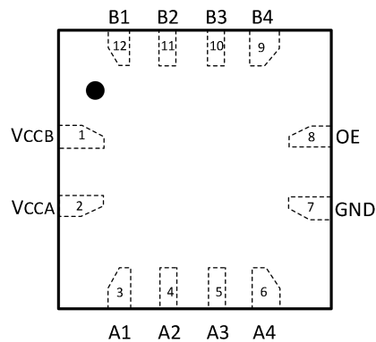
Fig.4-5. GT0104: QHC (QFN1.8×1.8-12L) Package
