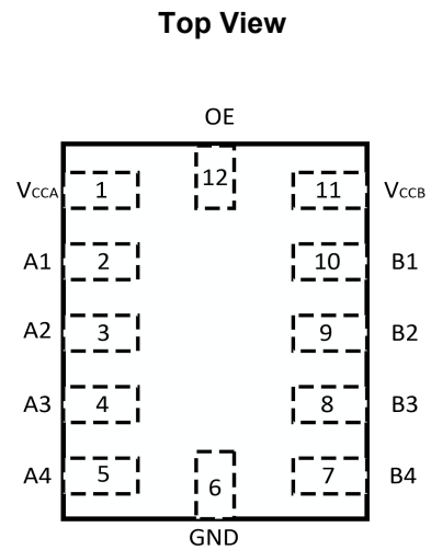
Fig.4-2. GT0104: SC (QFN2.0×2.0-12L) Package
