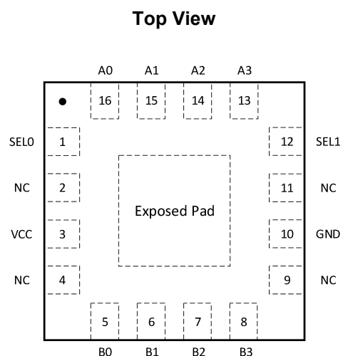
Fig.4-2.GT550: QSE (QFN3×3-16L) Package
