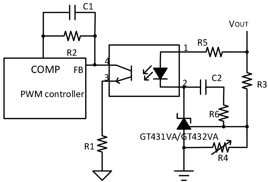
Fig.8-4. PWM Converter with Reference
