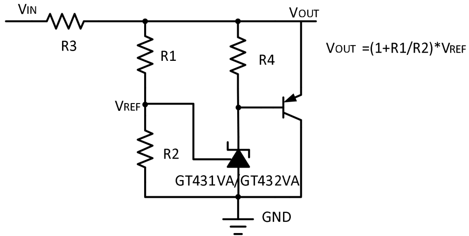
Fig.8-3. High Current Shunt Regulator
