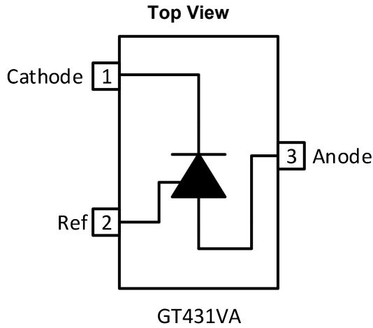
Fig.4-1. GT431VA: SOT23(3) Package
