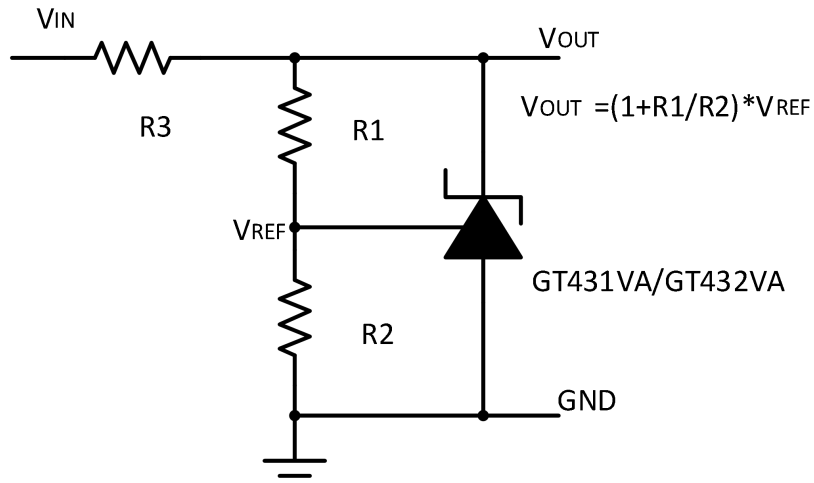
Fig.8-1. Shunt Regulator
