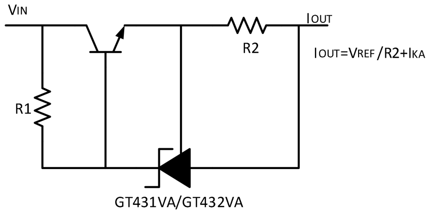
Fig.8-2. Current Source or Current Limit
