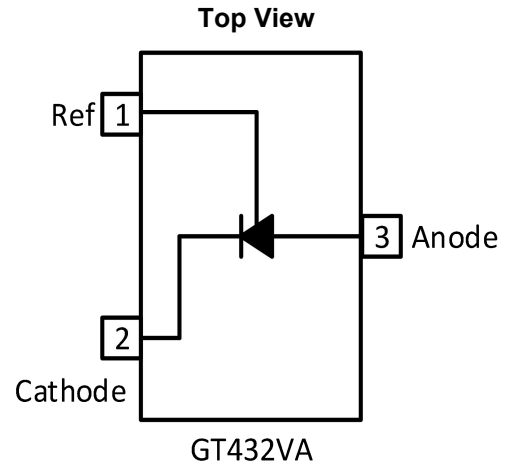
Fig.4-2. GT432VA: SOT23(3) Package
