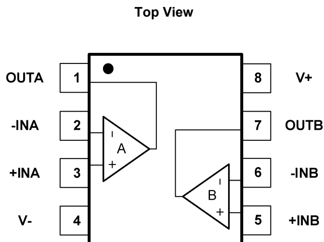
Fig.4-3.GT8102: M8(MSOP8) Package GT8102: T8(TSSOP8) Package GT8102: P8(SOP8) Package
