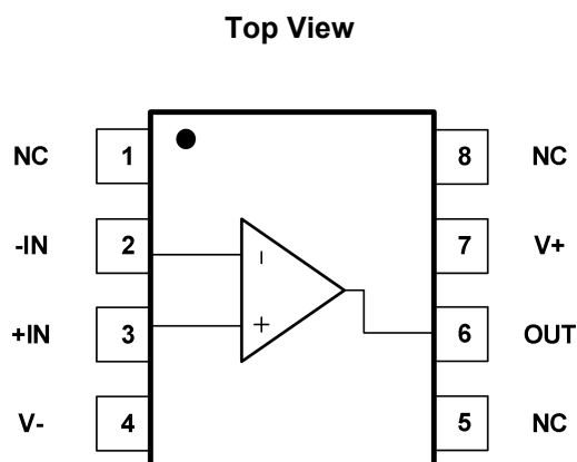
Fig.4-2. GT8101: M8 (MSOP8) Package GT8101: P8 (SOP8) Package
