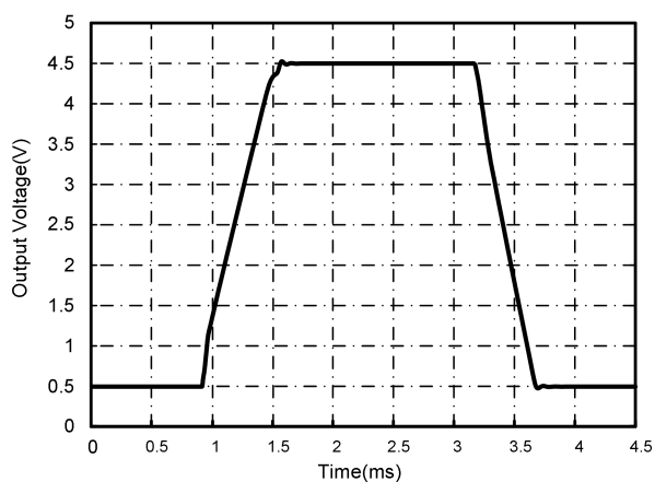
Fig.7-5. Large-Signal Step Response
