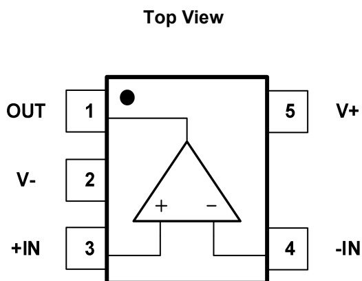
Fig.4-1. GT8101B: C5 (SC70-5) Package GT8101B: S5 (SOT23-5) Package
