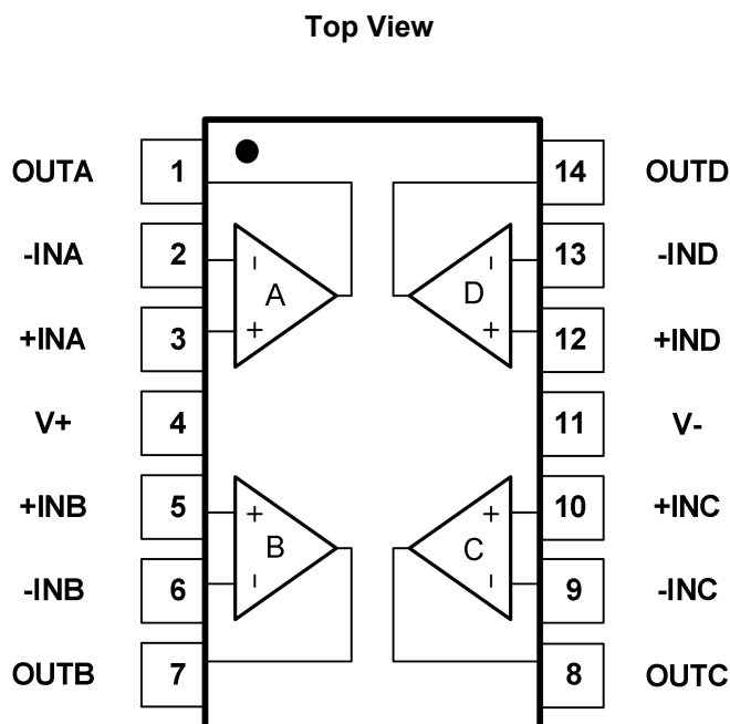
Fig.4-4. GT8104: TD (TSSOP14) Package
