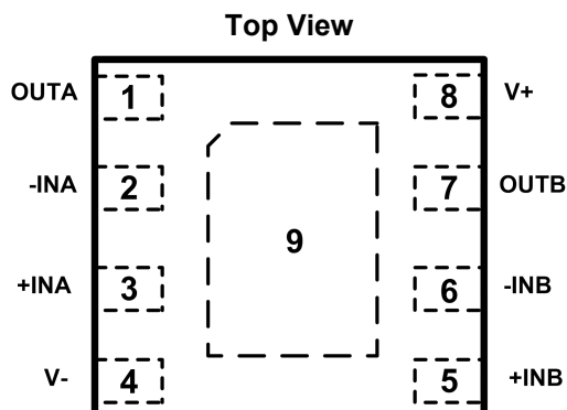
Fig.4-4. GT358: F8(DFN2*2-8L) Package
