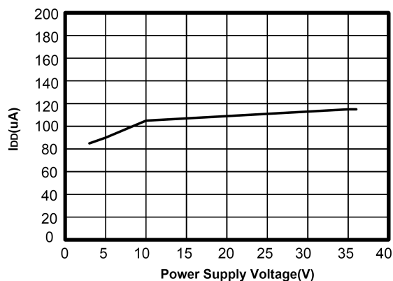
Fig.7-6. I_Q vs Power Supply Voltage(25°C)
