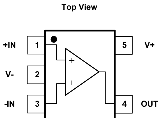
Fig.4-1. GT321: S5(SOT23-5) Package
