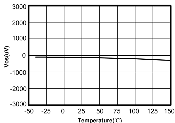
Fig.7-4. Offset Voltage vs Temperature
