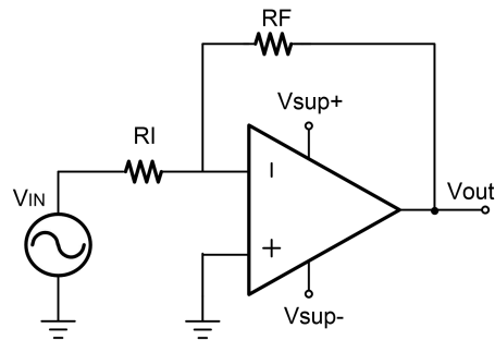
Fig.9-1. Dual-Supply Amplifier
