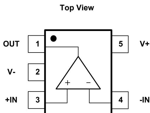
Fig.4-2. GT321B: S5(SOT23-5) Package
