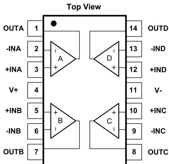
Fig.4-5. GT324: TD(TSSOP14) Package
