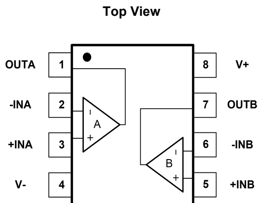
Fig.4-3. GT358: P8(SOP8) Package
