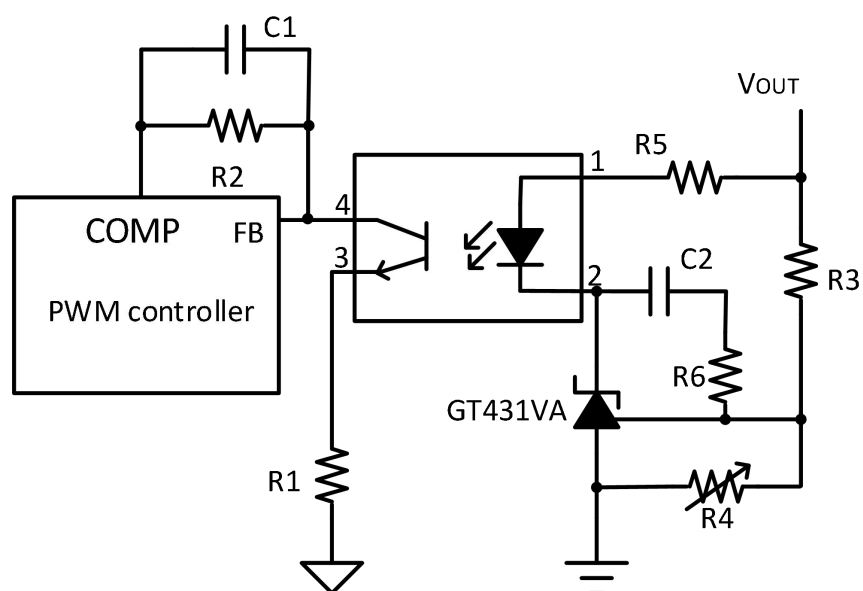
Fig.9-4. PWM Converter with Reference
