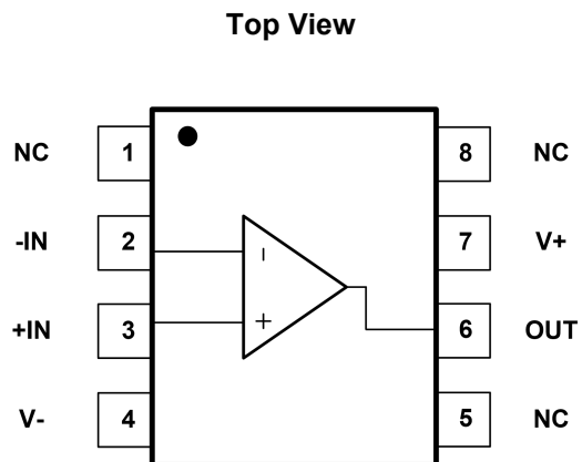
Fig.5-3. GT8341P: M8 (MSOP8) Package GT8341P: P8 (SOP8) Package
