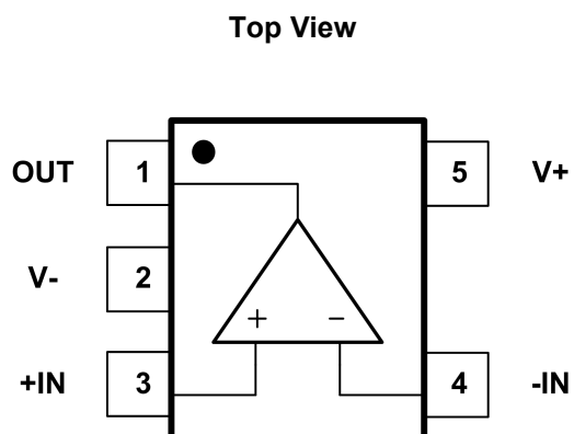
Fig.5-2. GT8341PB: C5 (SC70-5) Package GT8341PB: S5 (SOT23-5) Package
