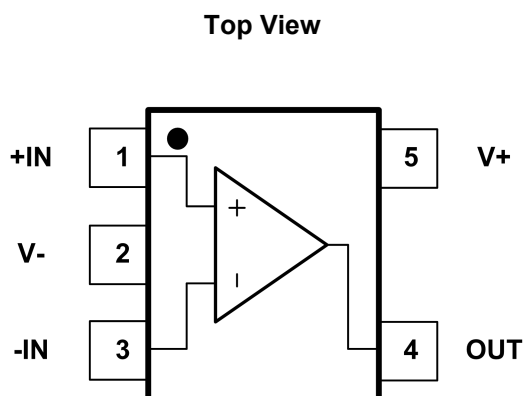
Fig.5-1. GT8341P: C5 (SC70-5) Package GT8341P: S5 (SOT23-5) Package
