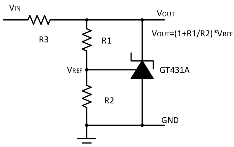
Fig.10-1. Shunt Regulator
