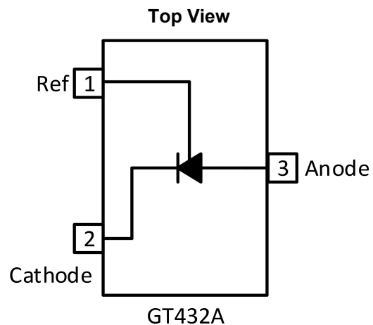
Fig.5-2. GT432A: SOT23(3) Package
