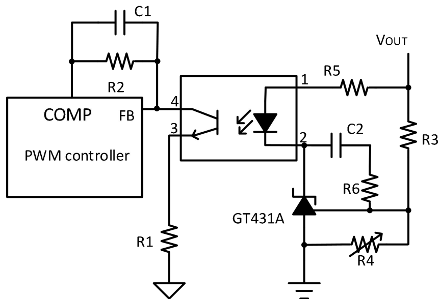
Fig.10-4. PWM Converter with Reference
