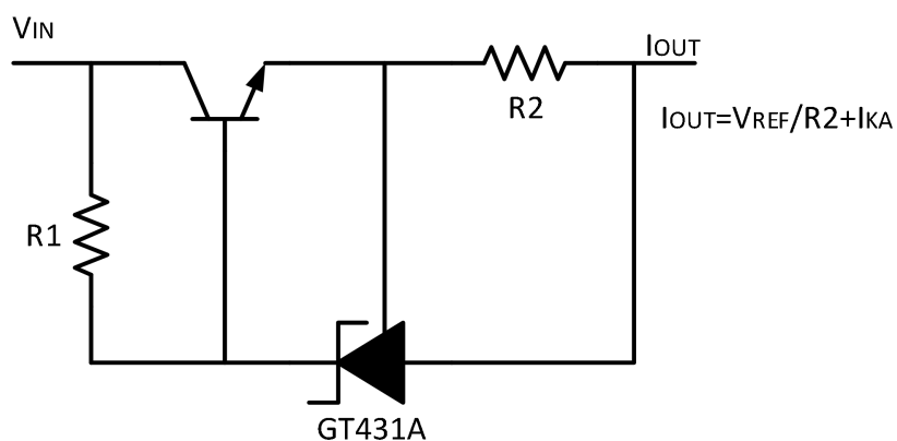
Fig.10-2. Current Source or Current Limit
