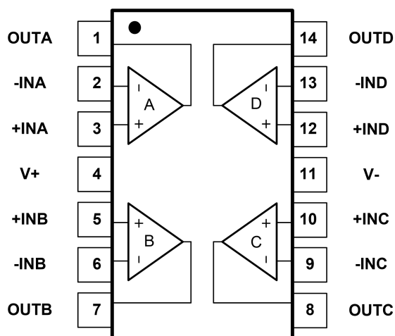
Fig.5-4. GT8324: TD (TSSOP14) Package GT8324: PD (SOP14) Package
