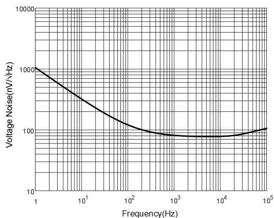
Fig.8-3. Voltage Noise vs Frequency
