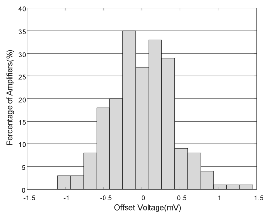
Fig.8-4. Offset Voltage Production Distribution
