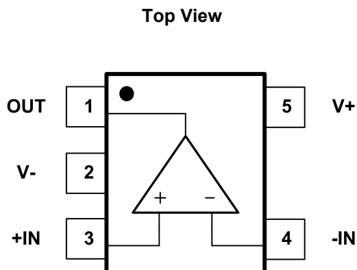
Fig.5-1. GT8321B: C5 (SC70-5) Package GT8321B: S5 (SOT23-5) Package
