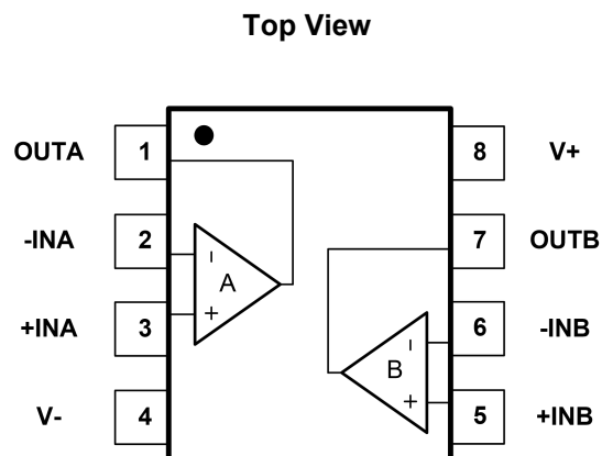
Fig.5-3.GT8322: M8(MSOP8) Package GT8322: P8(SOP8) Package
