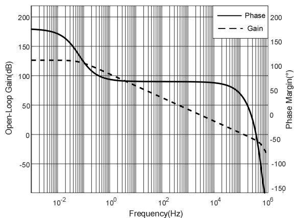
Fig.8-1. Open-Loop Gain and Phase vs Frequency
