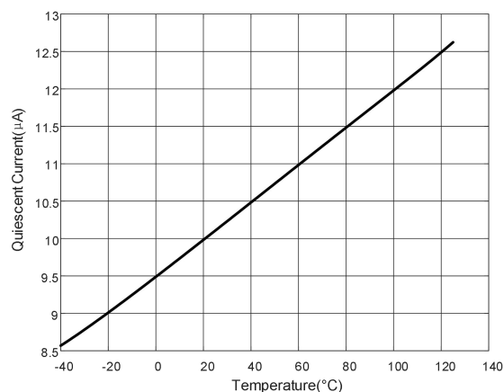
Fig.8-2. Quiescent Current vs Temperature
