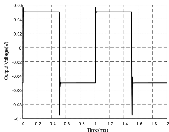
Fig.8-5. Small-Signal Step Response
