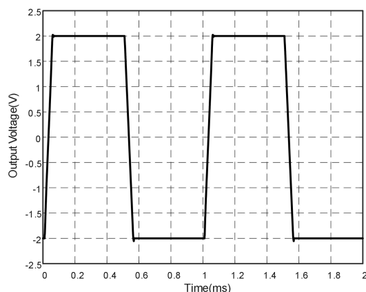
Fig.8-6. Large-Signal Step Response
