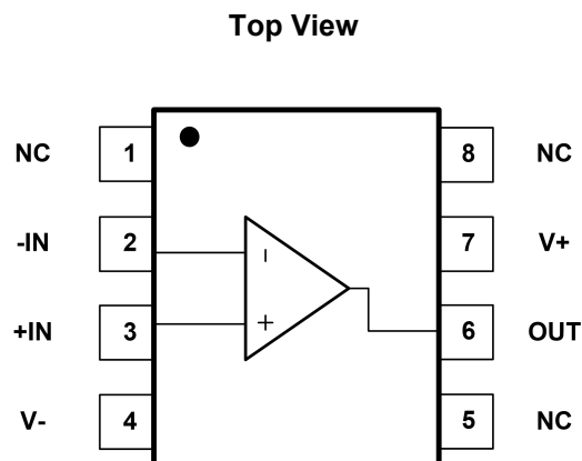
Fig.5-2. GT8321: M8 (MSOP8) Package GT8321: P8 (SOP8) Package
