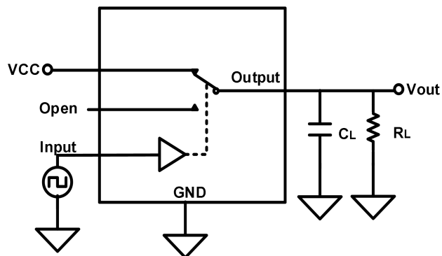
Fig.8-1. Turn-On ( t_{ON} ) and Turn-Off Time ( t_{OFF} )
