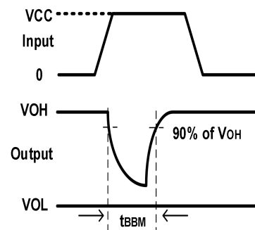
Fig.8-2. Break-Before-Make Time Delay ( t_{BBM} )
