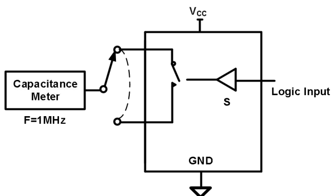
Fig.8-3. Channel ON/OFF Capacitance
