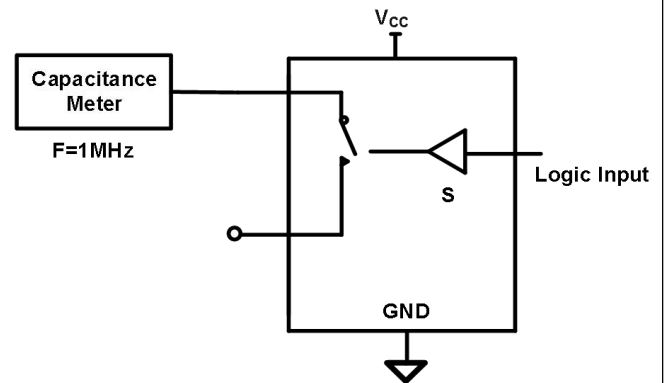
Fig.8-3. Channel ON/OFF Capacitance
