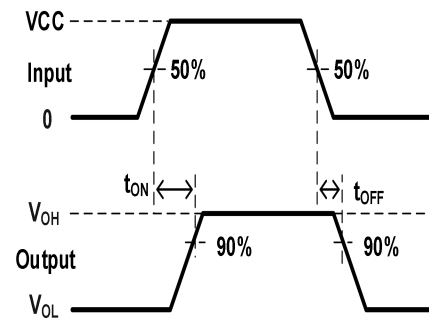
Fig.8-1. Turn-On ( t_{ON} ) and Turn-Off Time ( t_{OFF} )
