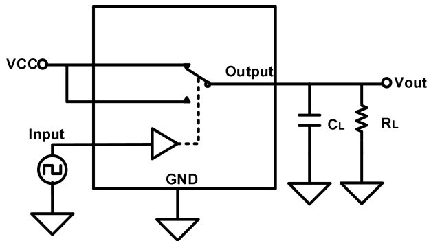
Fig.8-2. Break-Before-Make Time Delay ( t_{BBM} )
