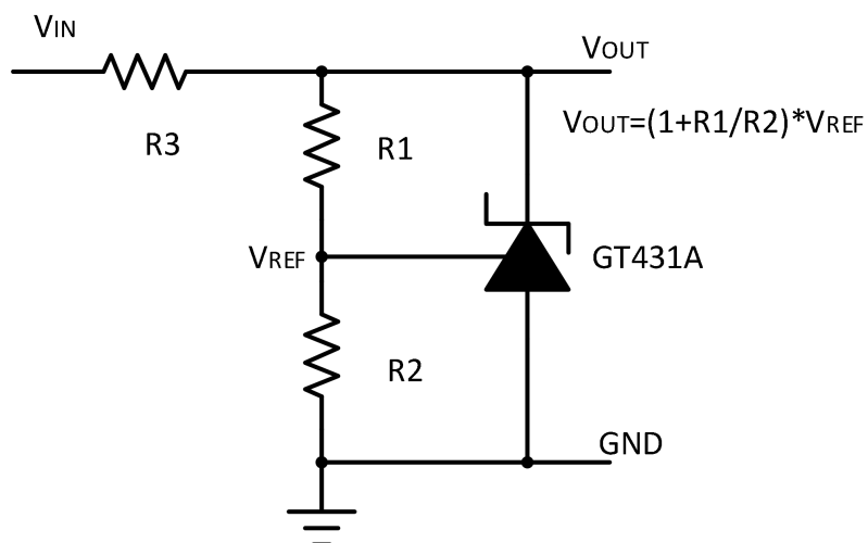
Fig.10-1. Shunt Regulator
