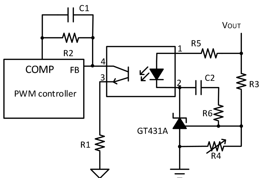
Fig.10-4. PWM Converter with Reference
