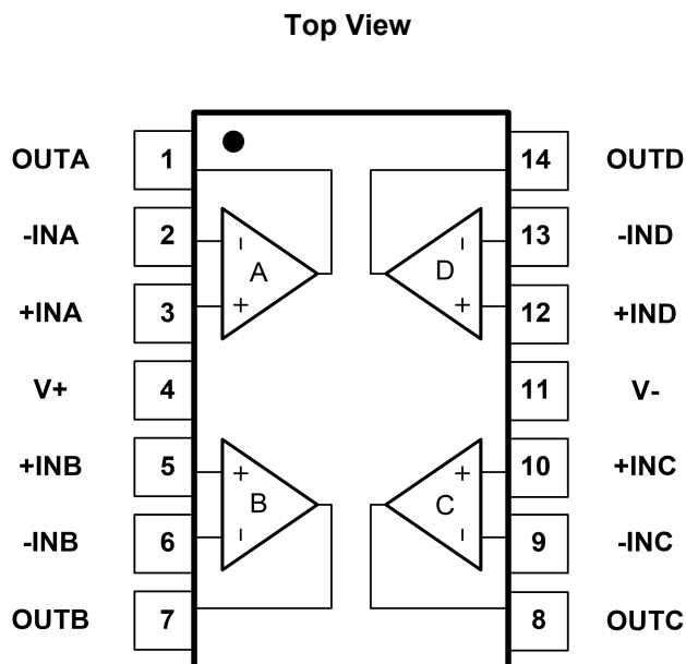
Fig.5-6. GT724: TD (TSSOP14) Package GT724: PD (SOP14) Package
