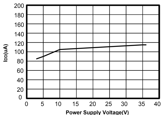
Fig.8-6. I_{QD} vs Power Supply Voltage(25°C)
