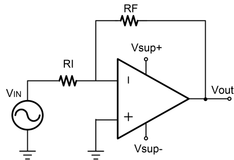
Fig.10-1. Dual-Supply Amplifier
