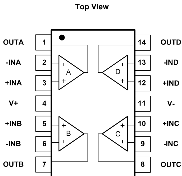
Fig.5-6. GT724P: TD (TSSOP14) Package GT724P: PD (SOP14) Package
