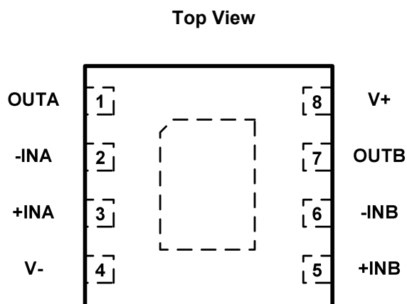
Fig. 5-5. GT722P: F8(DFN2*2-8) Package
