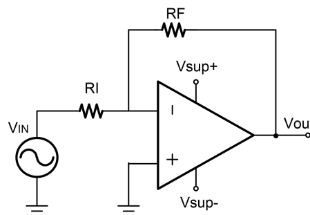
Fig.10-1. Dual-Supply Amplifier
