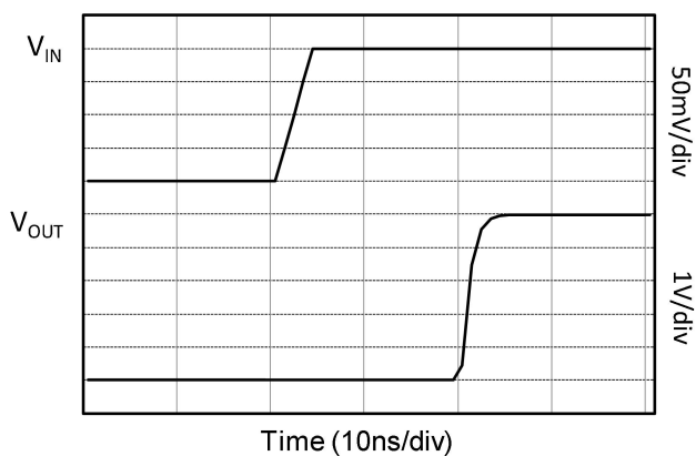
Fig.8-2. Propagation Delay (Low to High)
