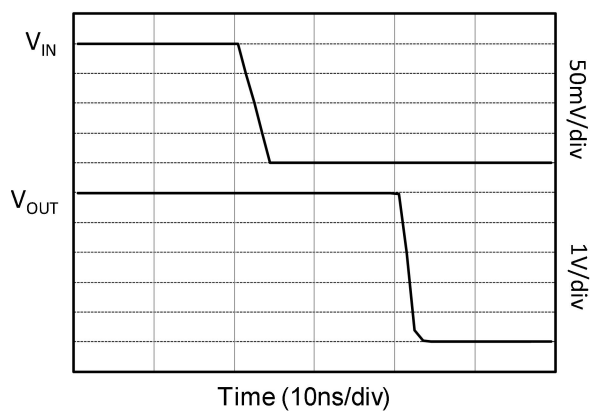
Fig.8-1. Propagation Delay (High to Low)
