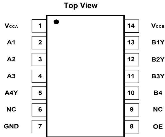
Fig.5-1. GTXU0304: TD (TSSOP14) Package
