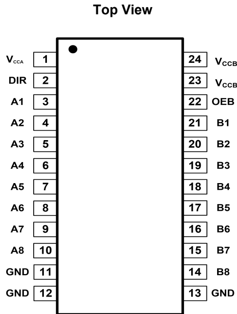
Fig.5-1. GT74LVC8T245: TH (TSSOP24) Package GT74LVC8T245: PH (SOP24) Package
