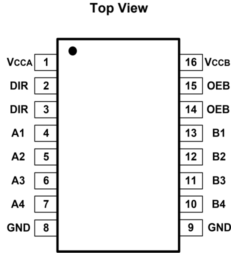
Fig.5-1. GT74LVC4T245: TE (TSSOP16) Package
