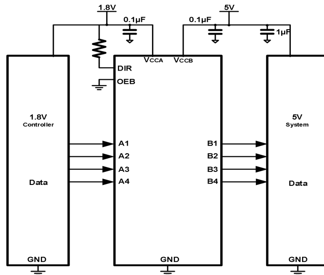
Fig.11-1. Typical Application Circuit
