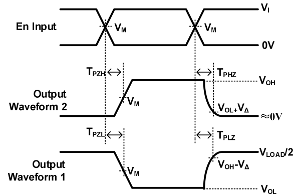
Enable and Disable Times Low-And High-Level Enabling
