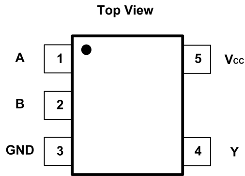
Fig. 5-1. GT74LVC1G86: S5 (SOT23-5) Package GT74LVC1G86: C5 (SC70-5) Package
